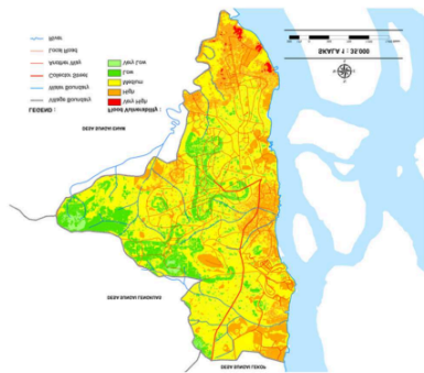
Fig. 12 Flood Vulnerability Map
