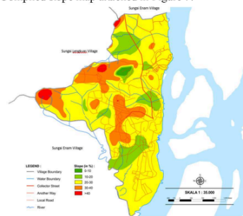
Fig. 7 Slope Map of Kijang Kota Village
