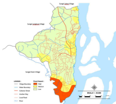
Fig. 11 Flood Hazard Map
