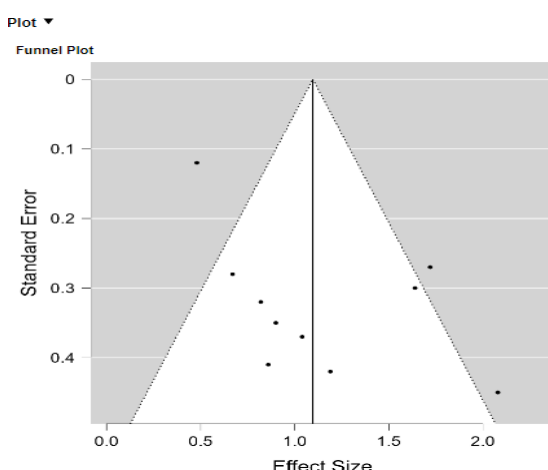
Figure 1. Funnel Plot Standard Error
