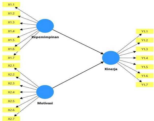
Gambar 2. Model PLS-SEM
