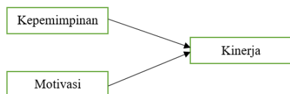
Gambar 1. Model Penelitian
