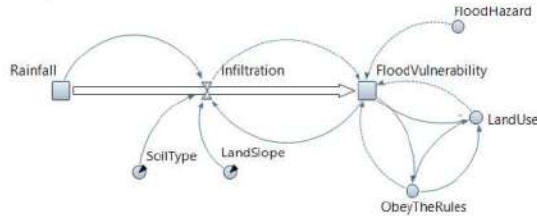
Fig. 5 Open Causal Flood Vulnerability Dynamical System Model
