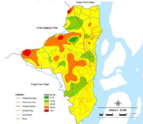
Fig. 7 Slope Map of Kijang Kota Village
