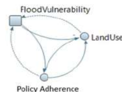
Fig.4 CLD of local regulations on disaster vulnerability
